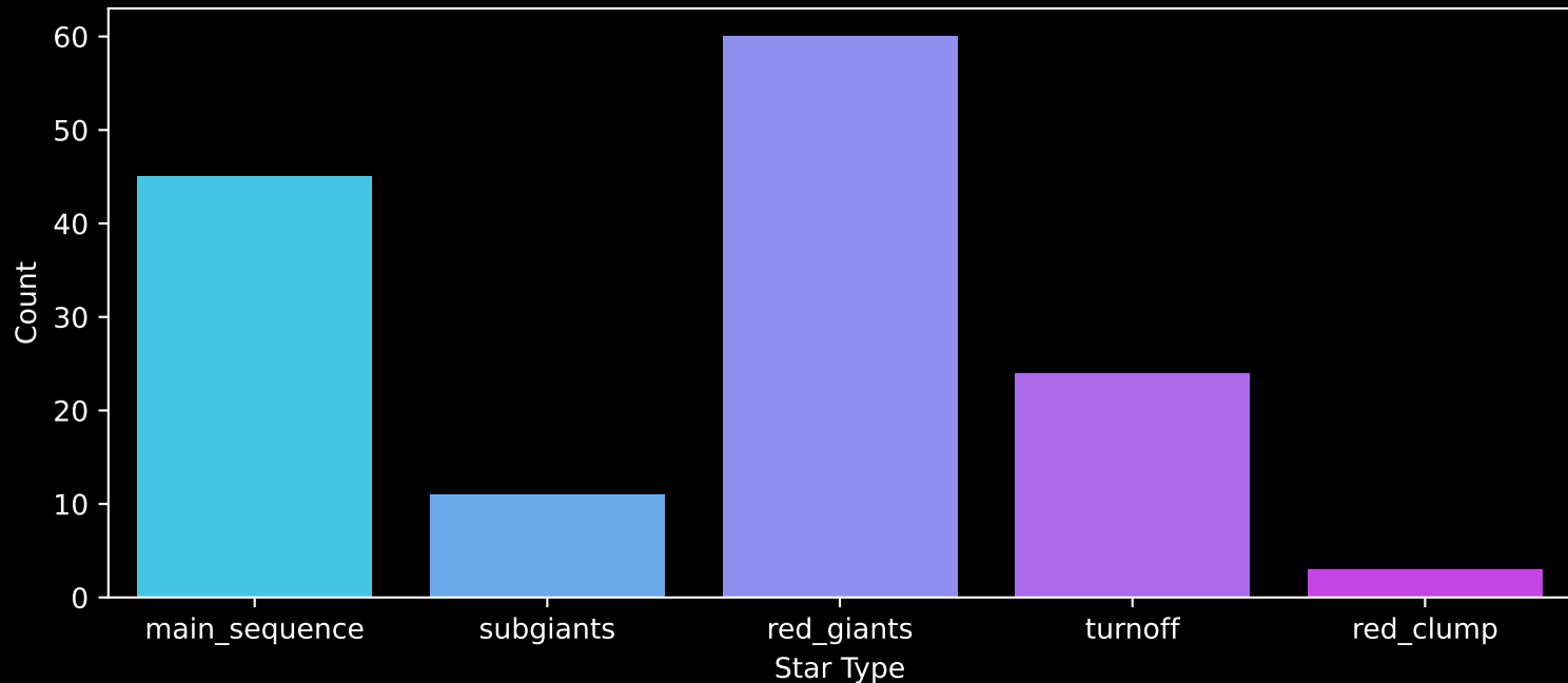
APOGEE DR17 Field: [349+22-O] Count plot of Star Type
