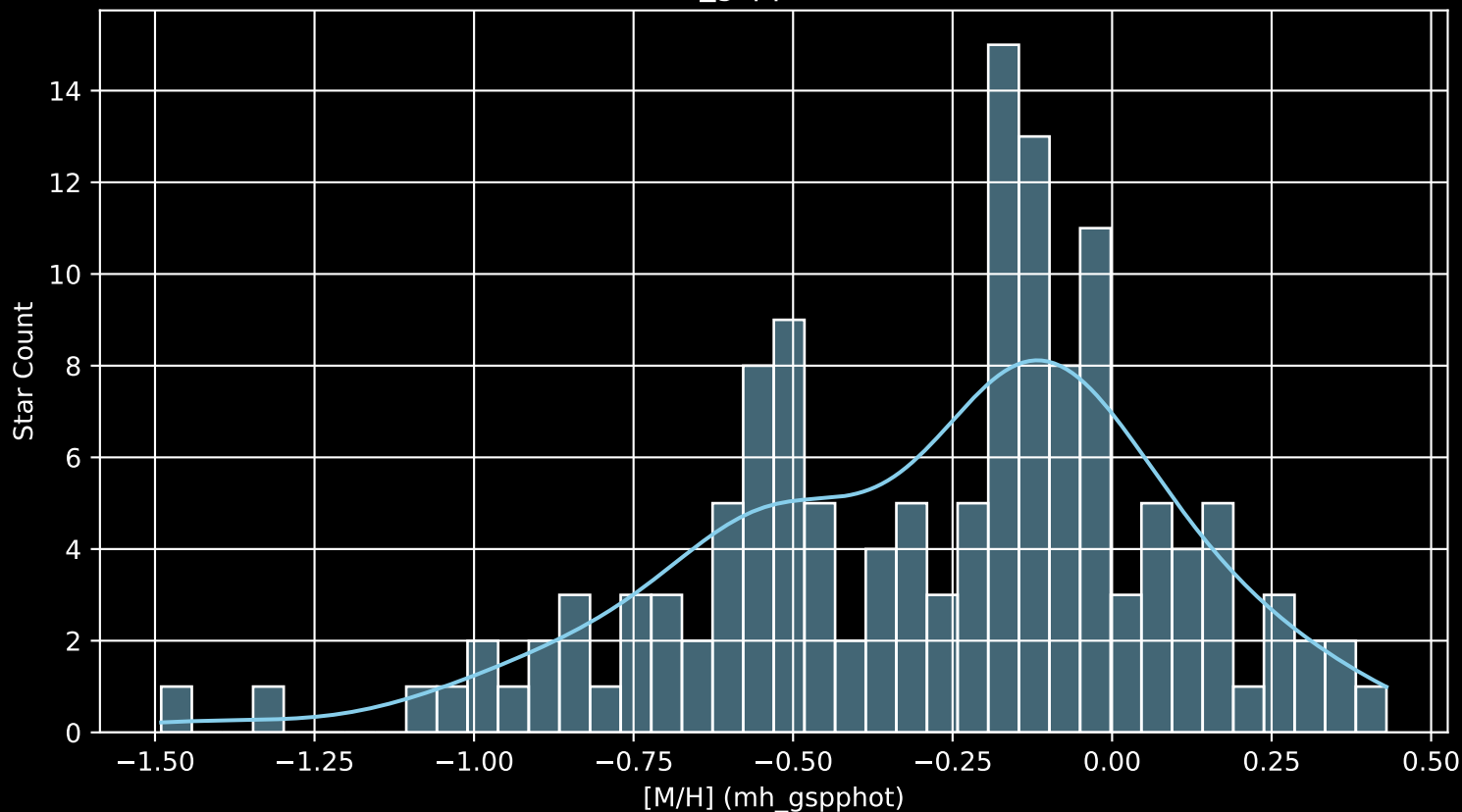
APOGEE DR17 Field: [349+22-O [M/H] (mh_gspphot) (n= 140)
