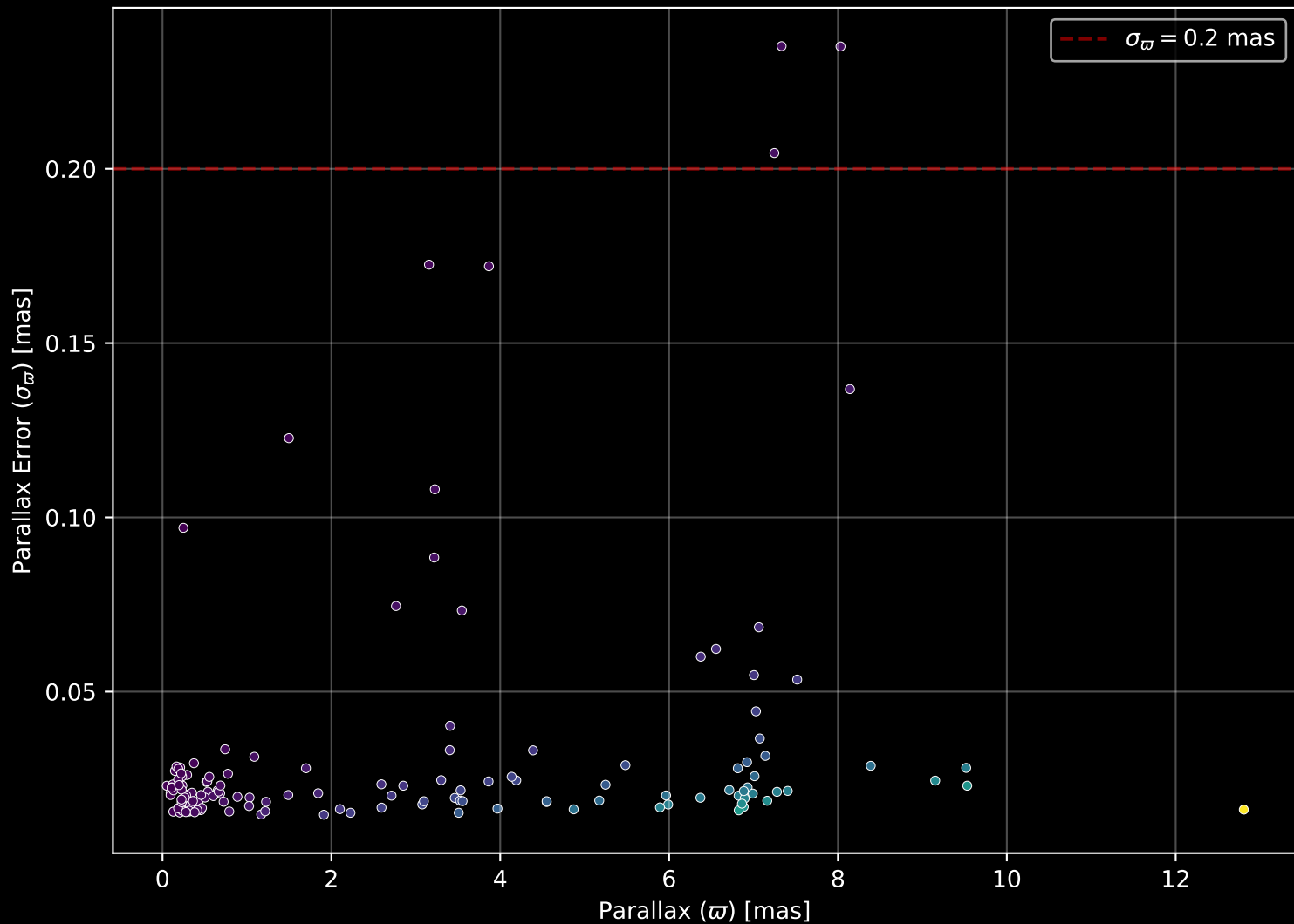
APOGEE DR17 Field: [349+22-O] Parallax Quality (n= 143)
