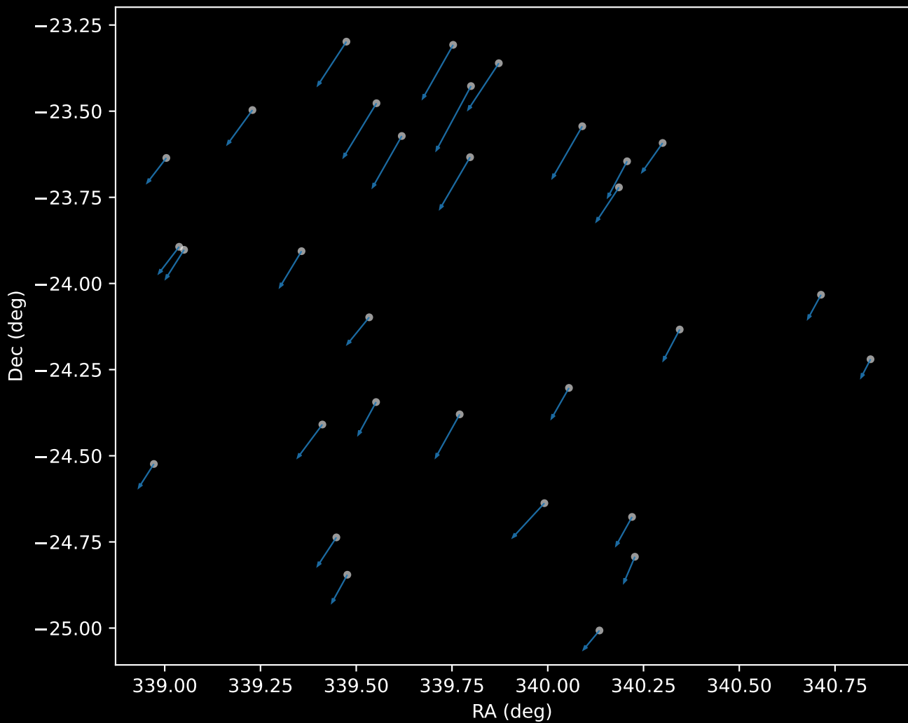
APOGEE DR17 Cluster 0 Proper Motion Vectors (n=31)
