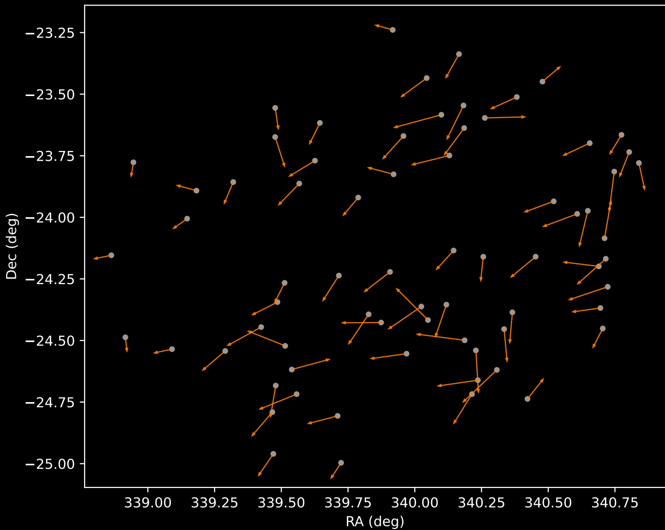
APOGEE DR17 Cluster 2 Proper Motion Vectors (n=70)
