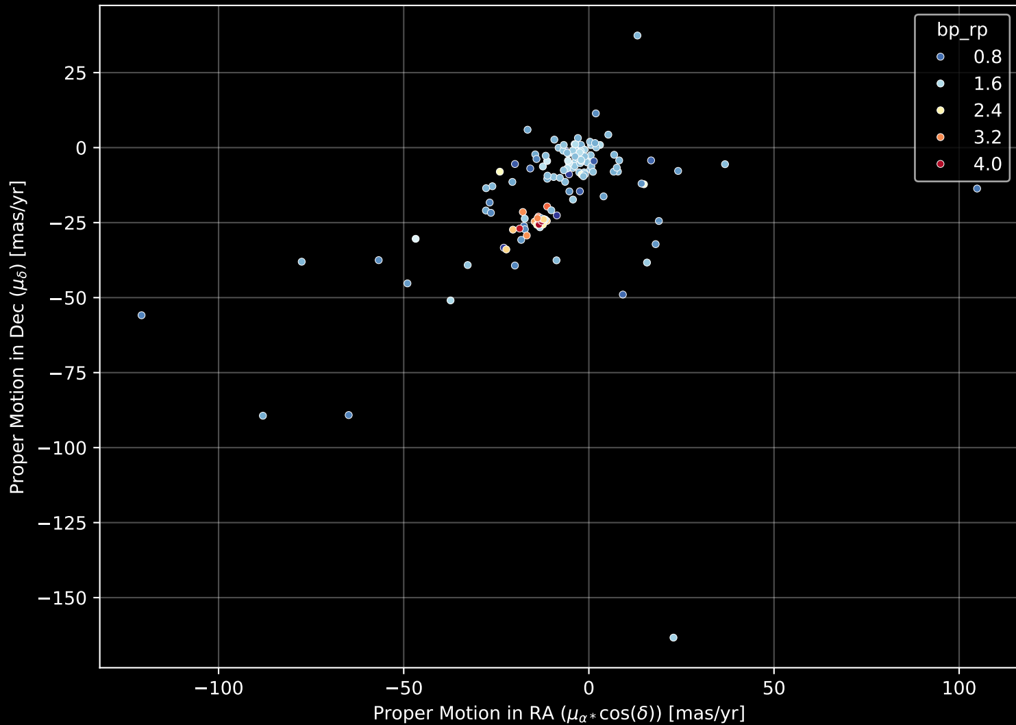
APOGEE DR17 Field: [349+22-O] Proper Motion Diagram (n= 143)
