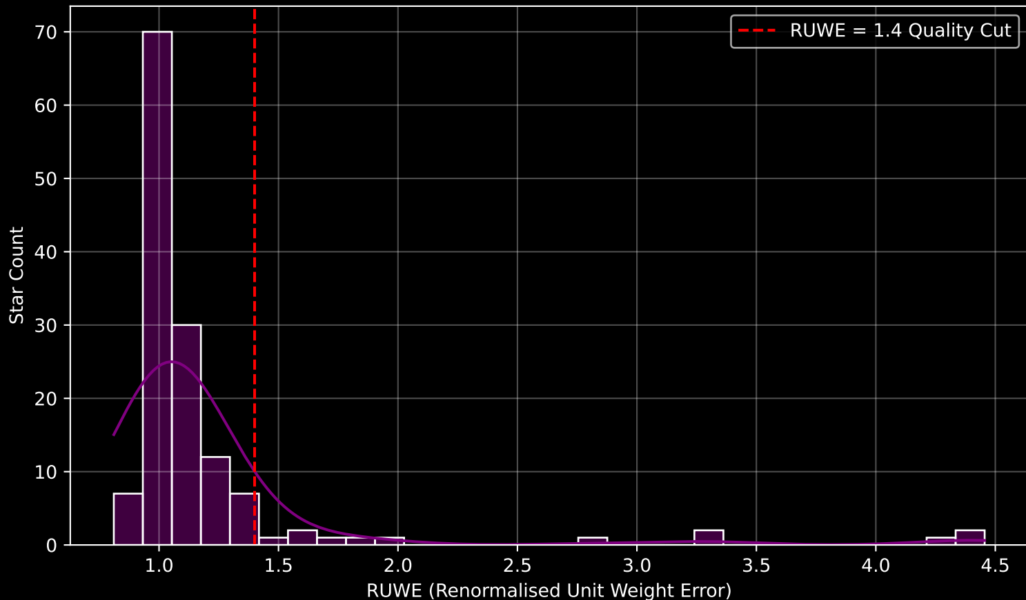
GAPOGEE DR17 Field [349+22-O] RUWE Distribution (n= 138)
